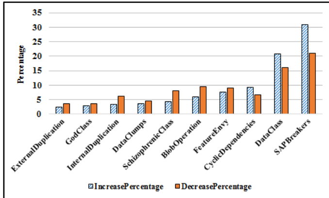
Fig. 10. Breakdown of smells introduced and removed
