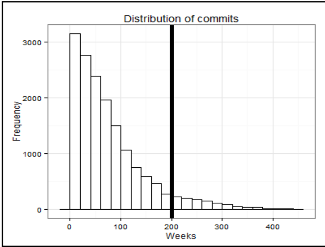
Fig. 1. Distribution of commits over time (vertical line indicating cutoff at 200 weeks)
